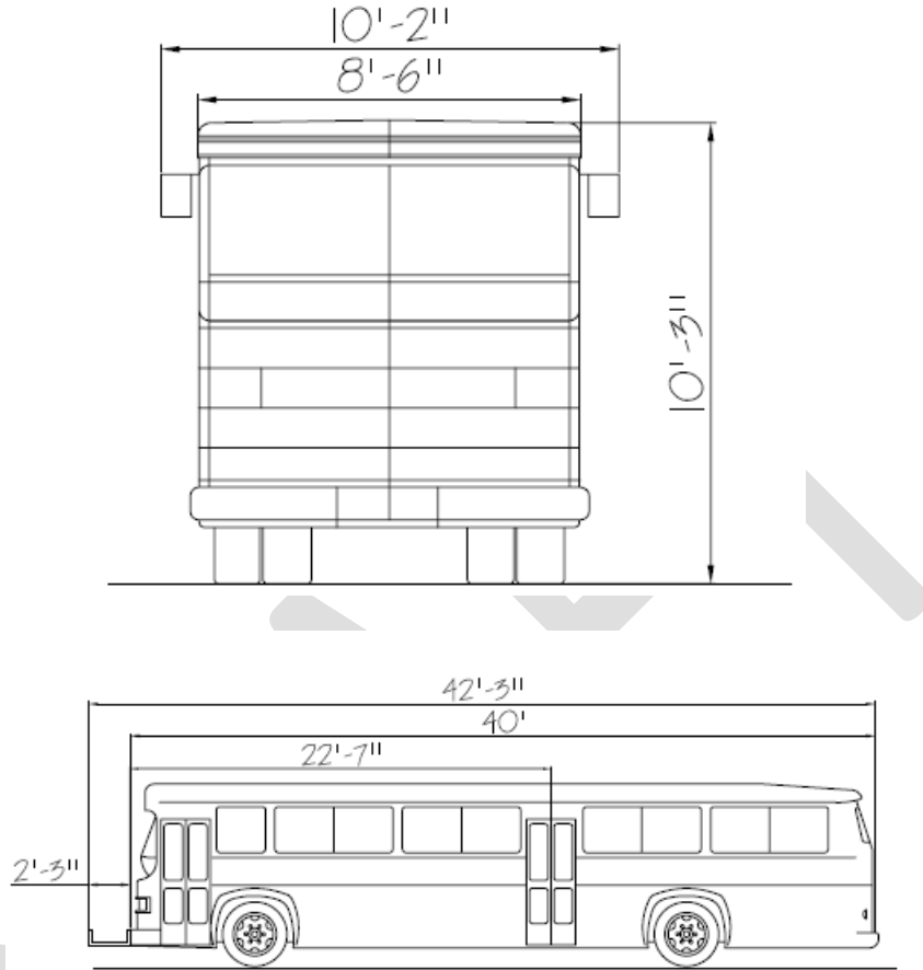
Exhibit 1: Standard 40-foot bus dimensions
