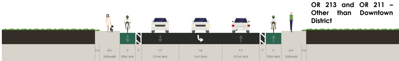
Arterial with Buffered Bike Lanes and Center Turn Lane (68-foot ROW, 52-foot Paved Width)
