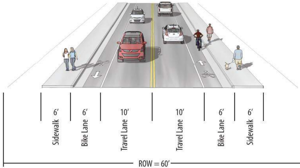
Figure 4C. Local Cross section Option C
