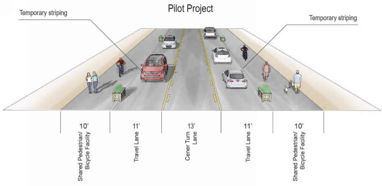
Figure 24. Pilot Project (above) rendering and (below) cross section
