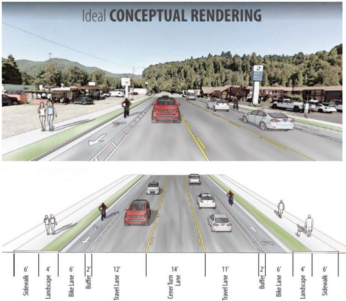
Figure 25. Conceptual Ideal Cross section Design (above) rendering and (below) cross section
