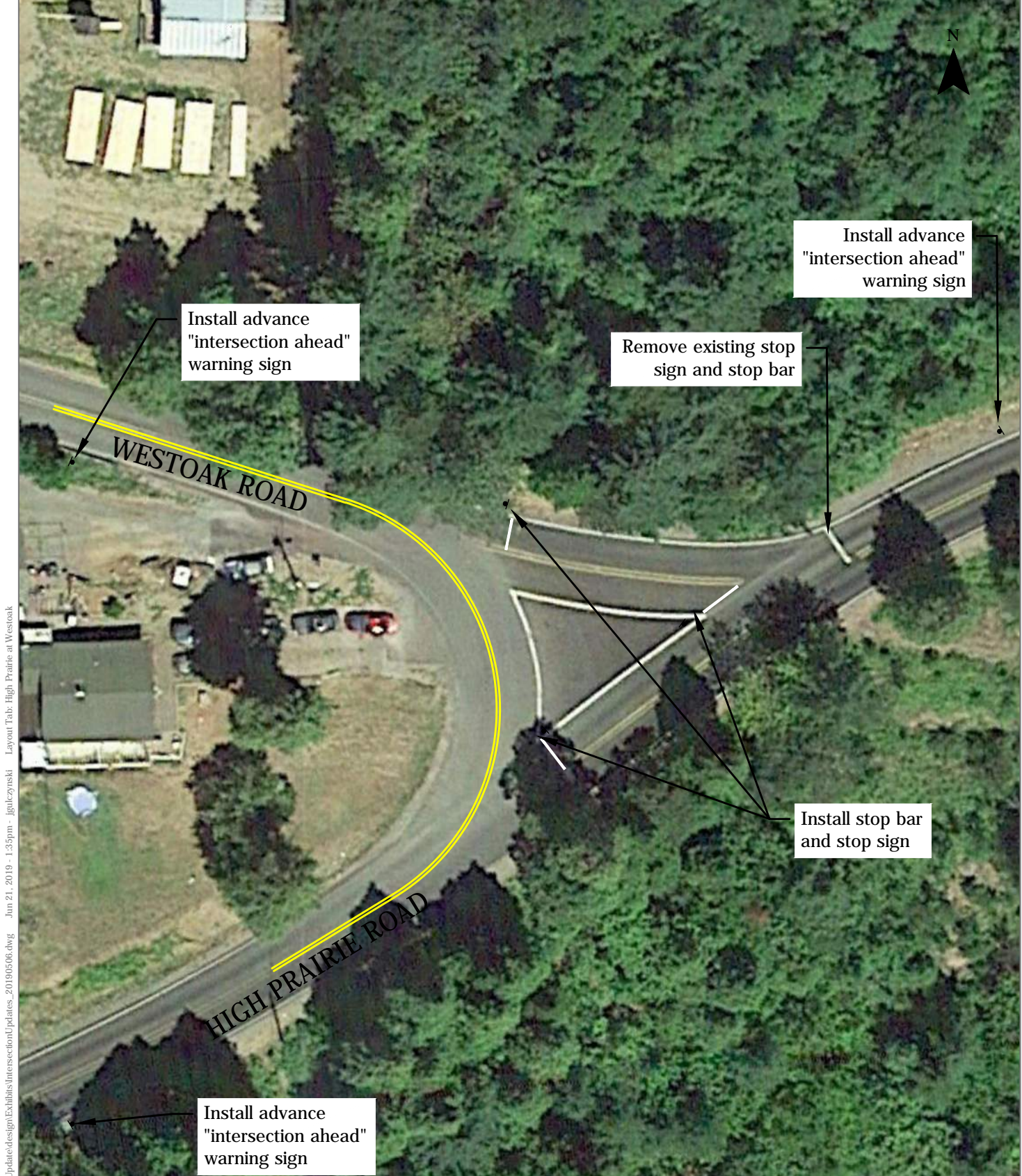
Intersection Safety Improvement at High Prairie Road/Westoak Road Oakridge, Oregon
