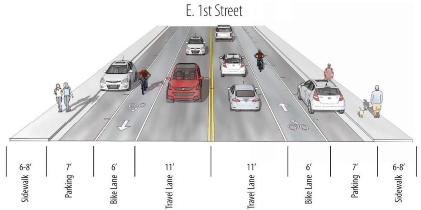
Figure 7. Proposed E 1 st Street Cross Section between Hazel Street and Beech Street
